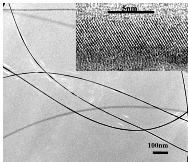
Figure 1. A TEM image of GeNWs grown from \sim 5 \text{ nm} Au nanoparticles. Inset: A high-resolution TEM image of a GeNW with a diameter of \sim 4 \text{ nm} .
